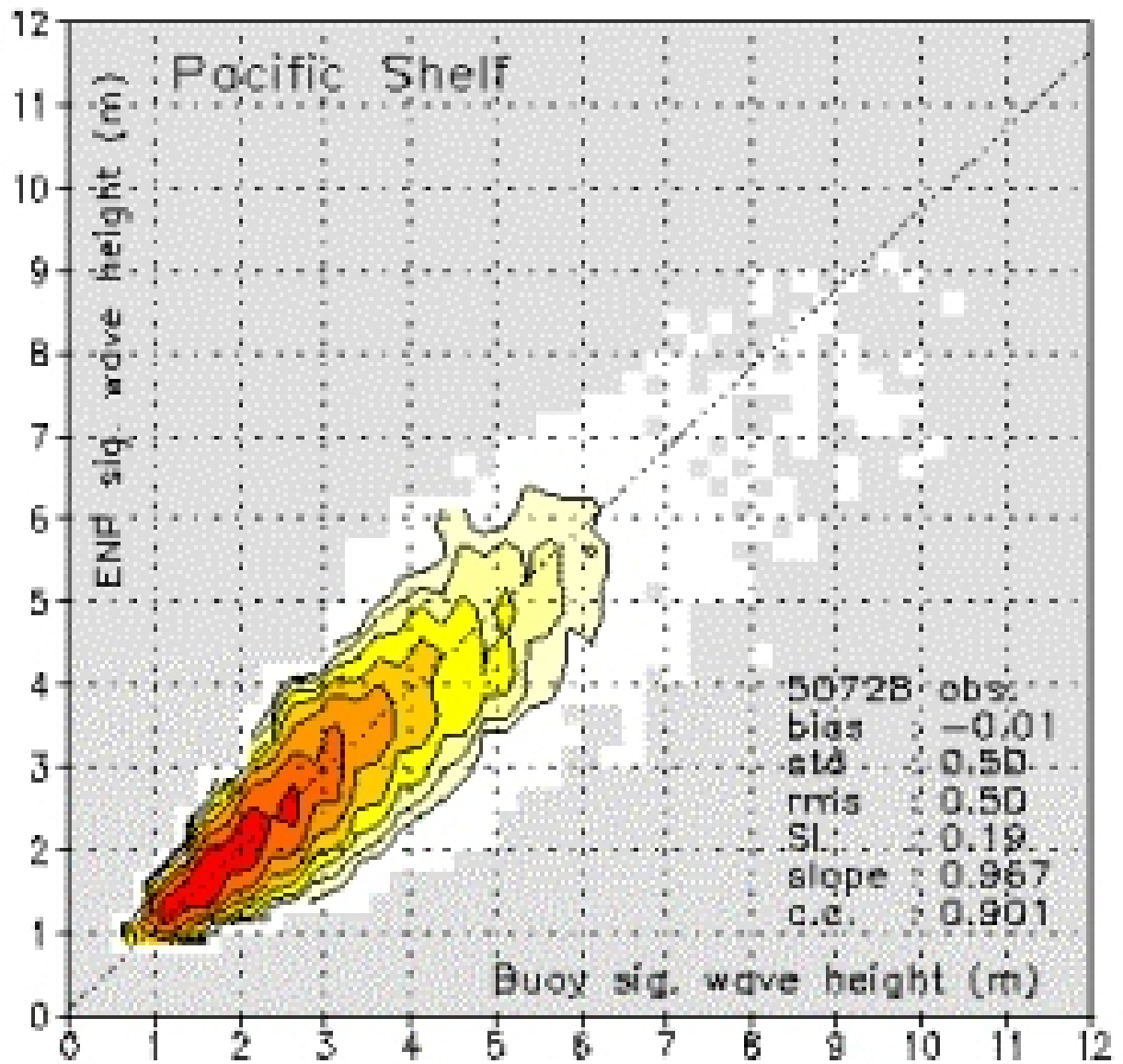
Figure 7. Statistical evaluation of ENP hindcast against buoy measurements along the shelf of the West coast.
