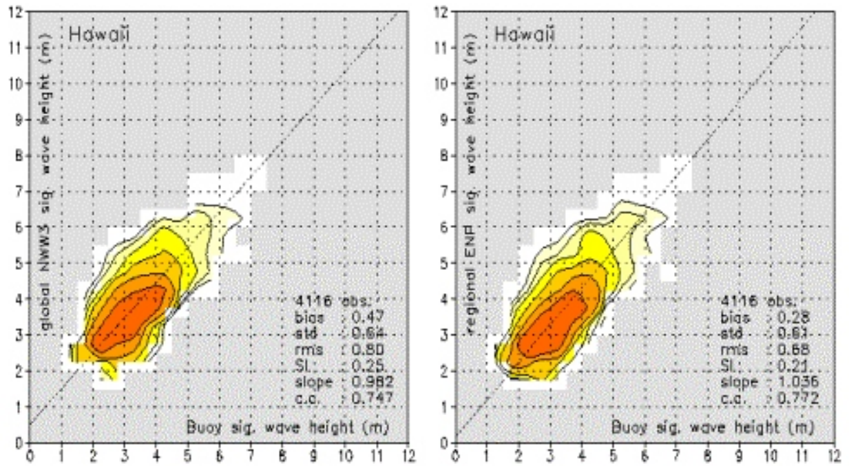
Figure 4. Scatter plots comparing hindcasts of significant wave heights for the NWW3 (left) and the ENP (right) for the months of December 2001 and January 2002.
