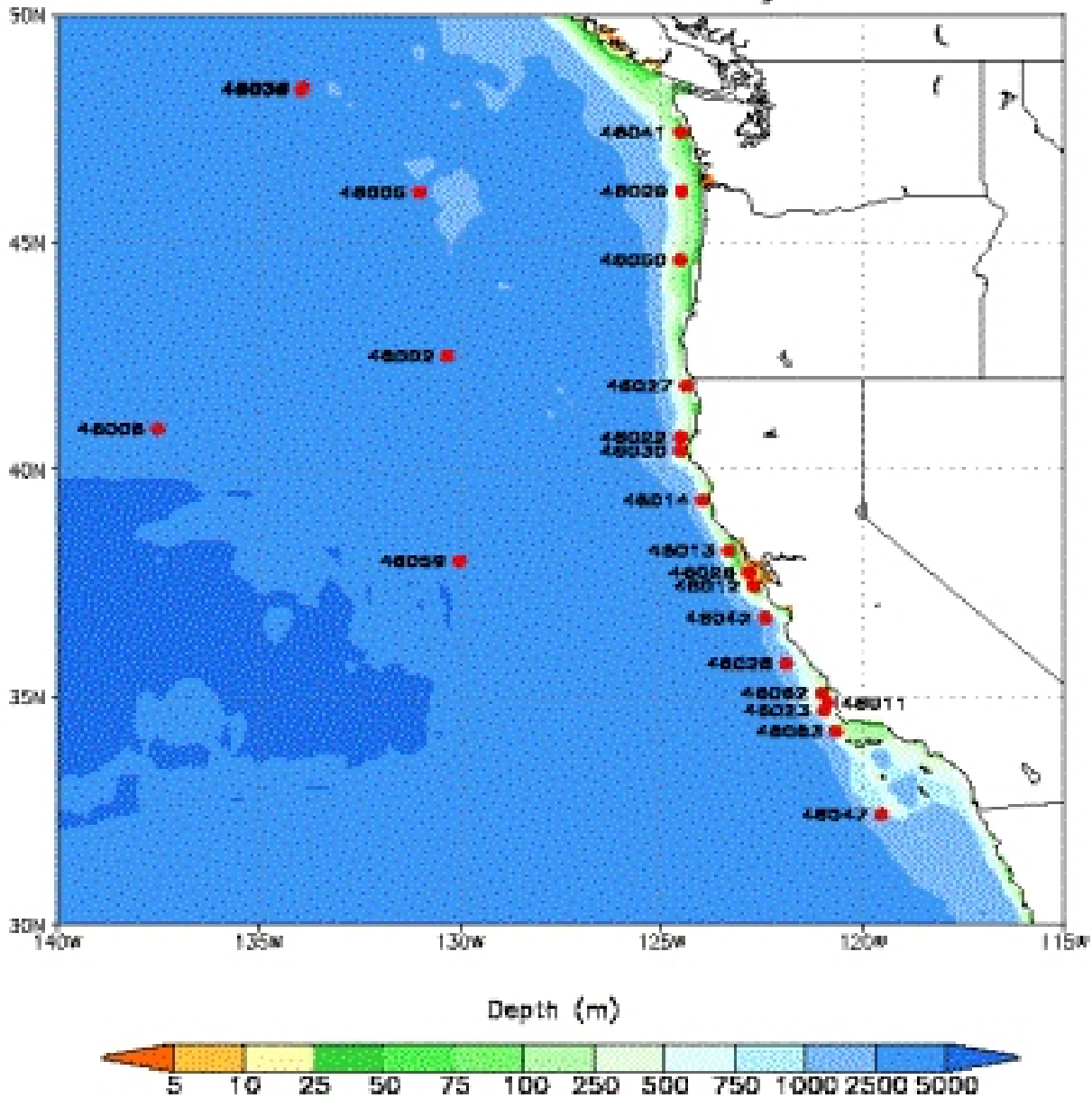
Figure 6. Available buoy measurements off and along the West coast of the U.S.
