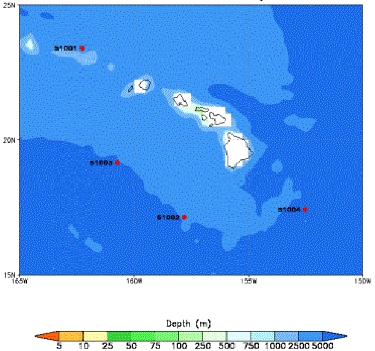
Figure 3. Locations buoys used to verify ENP model output in the vicinity of the Hawaiian Islands.
