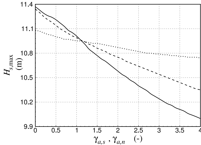
Fig. 6. Maximum wave height H_{s,max} (solid line) corresponding to the test case of Fig. 5 as a function of the smoothing parameters \gamma_s and \gamma_n in Eq. (12), p = 0 . (Dashed and dotted lines) corresponding results for spatial grid resolution increased from 25 km to 12.5 and 6.25 km, respectively.
